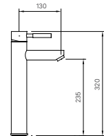
BFV-8000S | BFV-8000S-1C | BFV-8000S-5C
