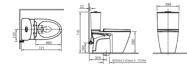
AC-504VAN | C-504VAN | AC-504VWN | C-504VWN
